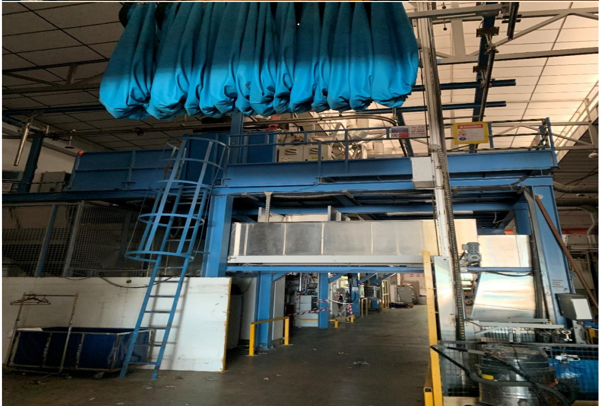
Jensen SenKing Continuous Batch Washer System 2016
